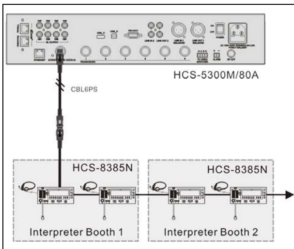
Figure 2.4 Connecting to HCS-8385N
