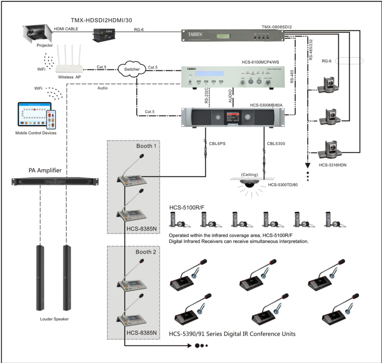
Figure 2.11 System connection [Wireless discussion + video tracking + central control]
