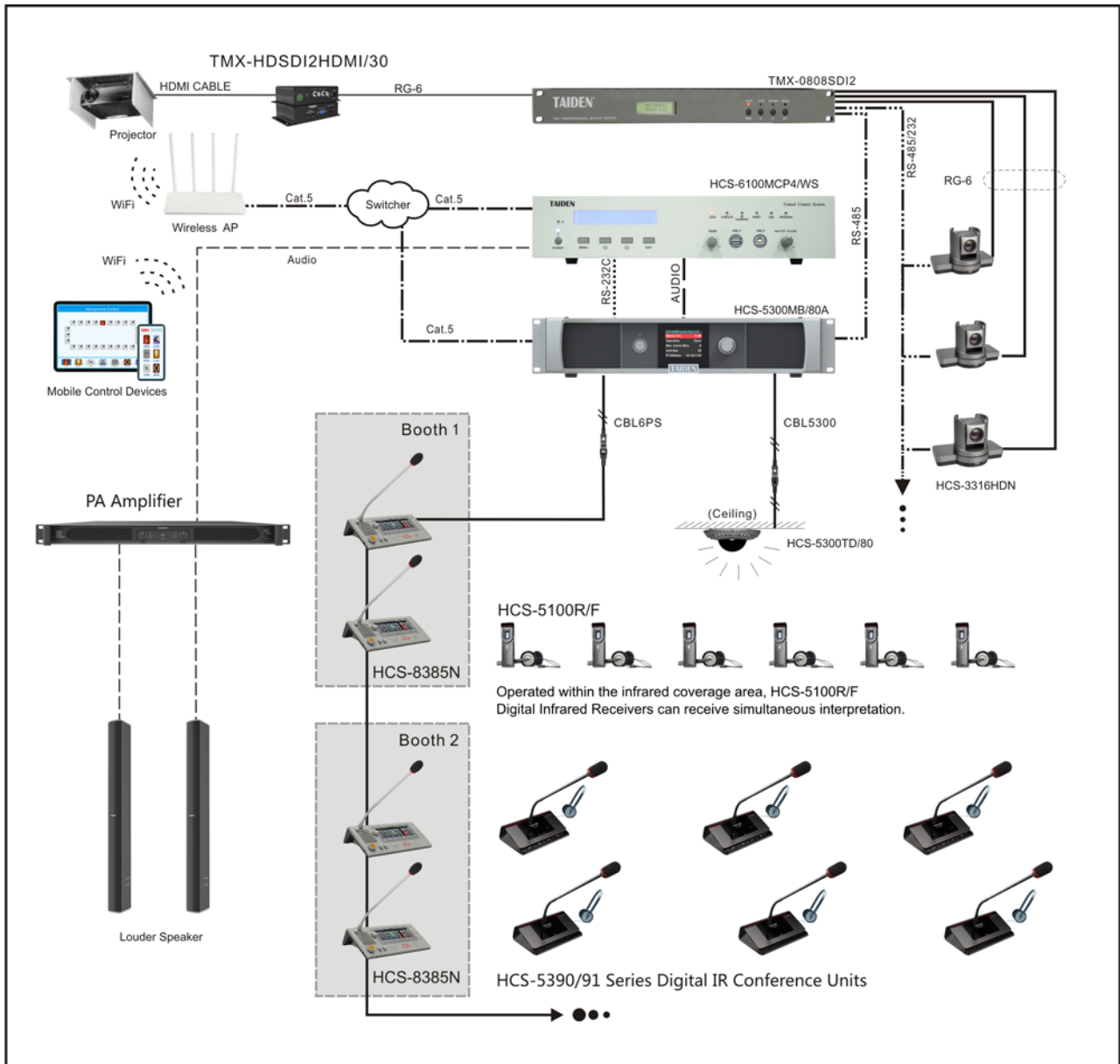
Figure 2.10 System connection [Wired/wireless discussion + digital simultaneous interpretation + video tracking + central control]
