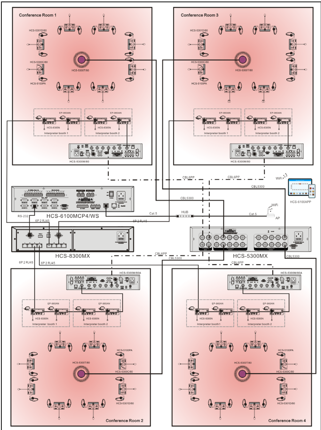
Figure 6.3 Conference rooms combination 2
