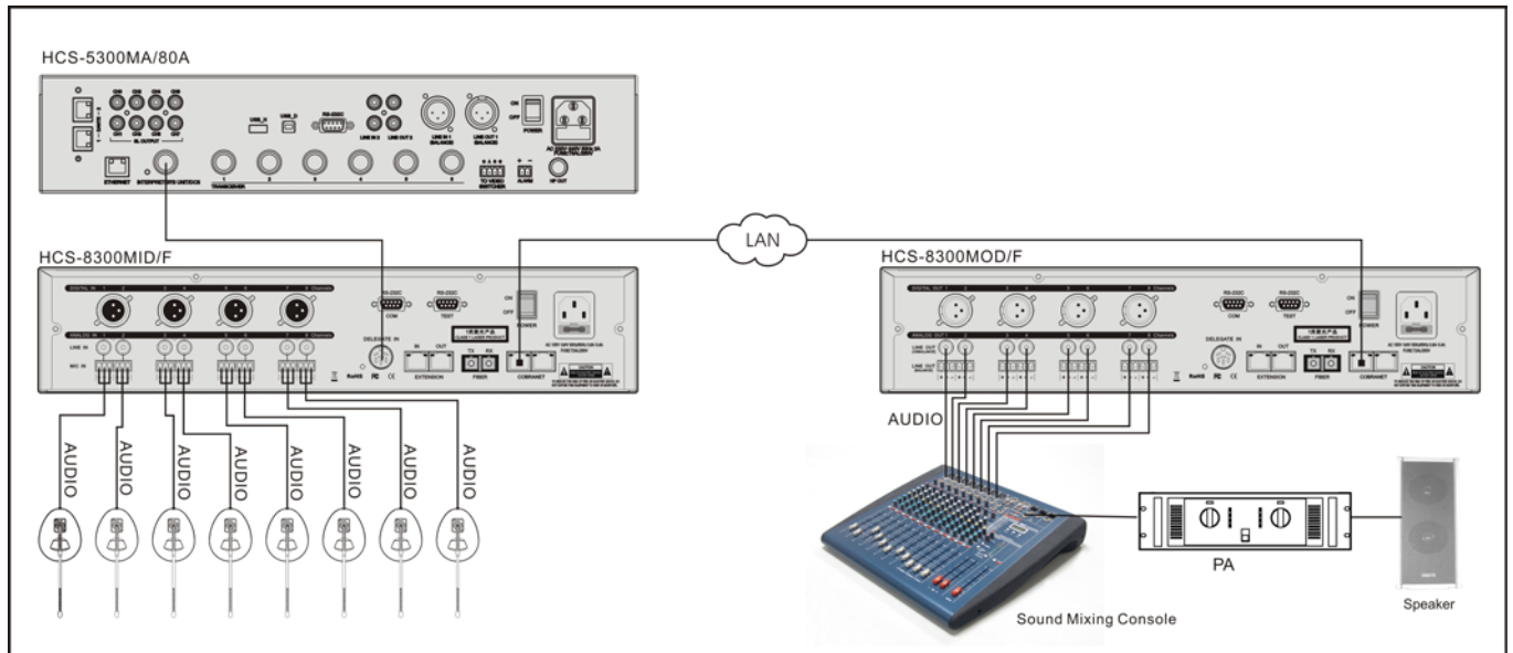
Figure 2.9 HCS-5300M+HCS-8300MI+HCS-8300MO multi-channel digital audio transmission solution
