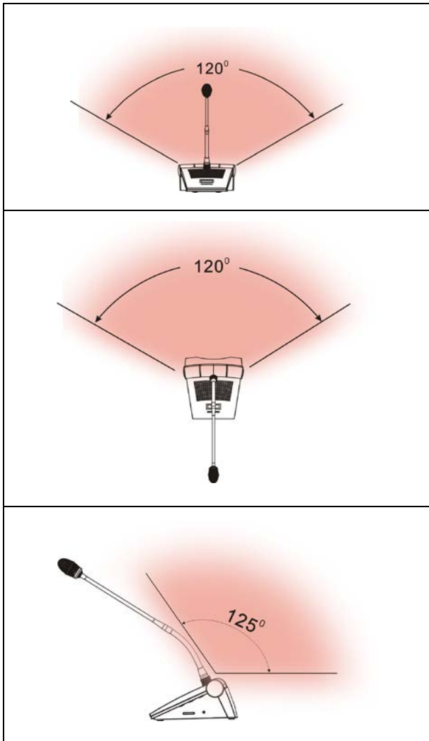
Figure 4.10 Coverage area of digital infrared wireless conference unit
