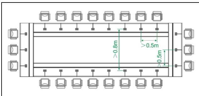
Figure 4.24 Distance between conference units
