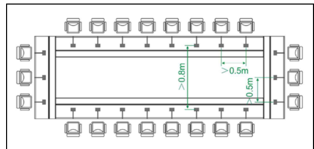
Figure 4.18 Distance between conference units
