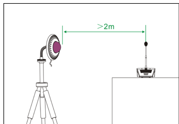
Figure 4.13 Distance between conference unit and transceiver
