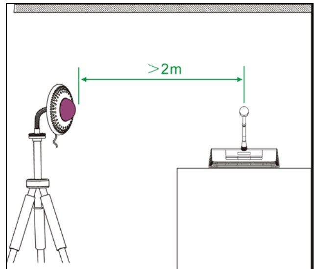
Figure 4.25 Distance between conference unit and transceiver
