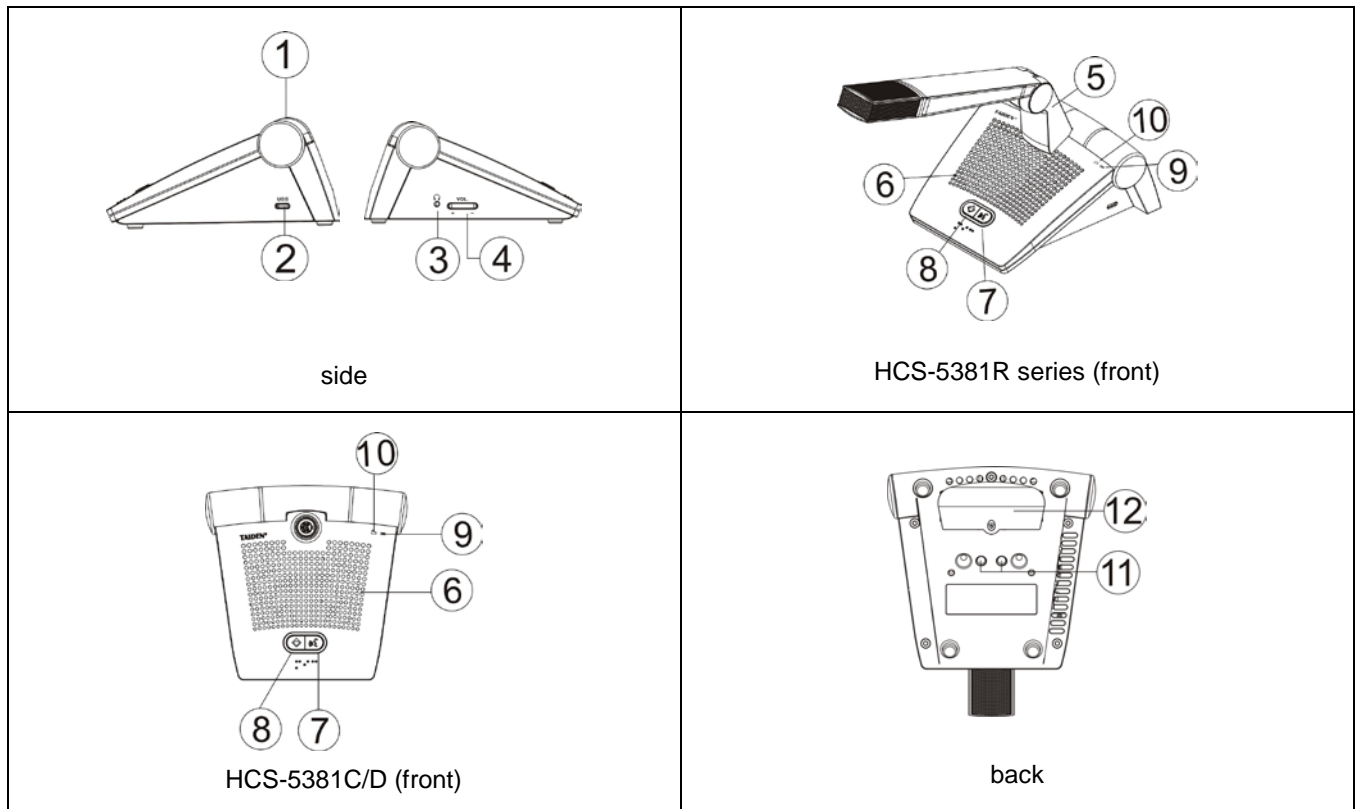
Figure 4.15 HCS-5381 series digital infrared wireless conference unit
