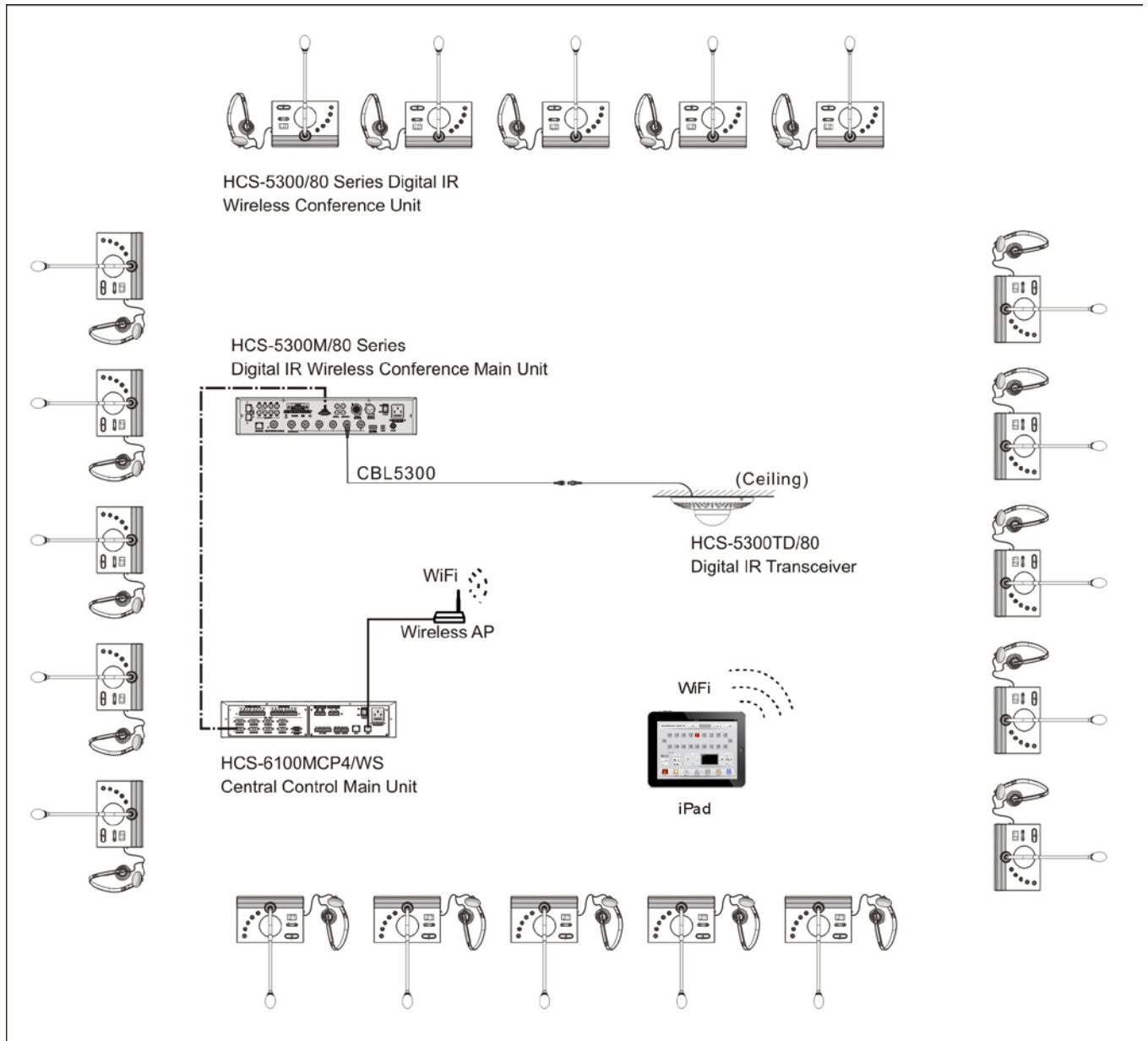
Figure 1.1 System overview
