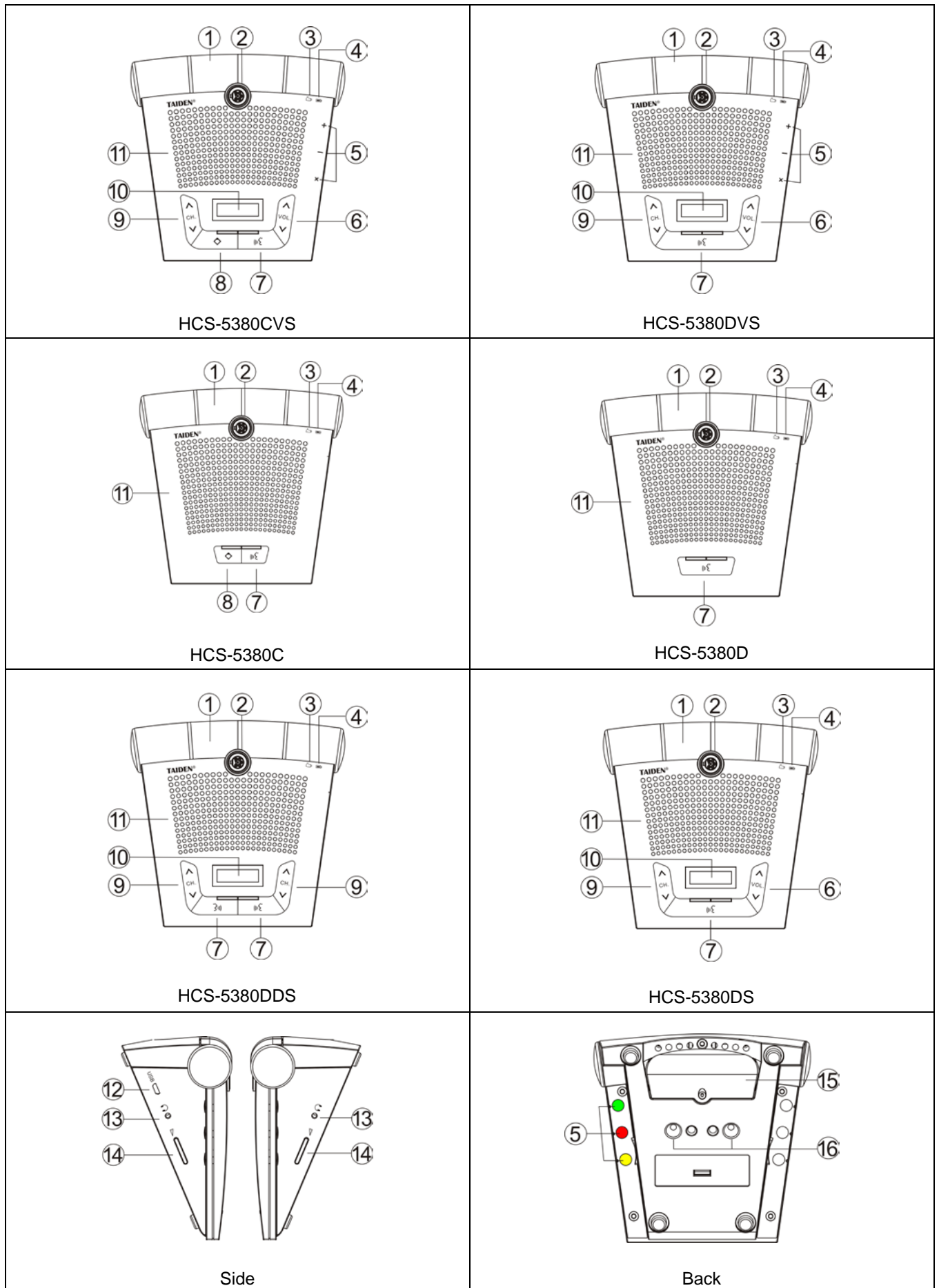
Figure 4.9 HCS-5380 series digital infrared wireless conference unit
