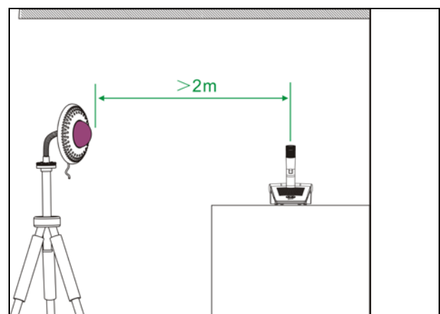
Figure 4.19 Distance between conference unit and transceiver
