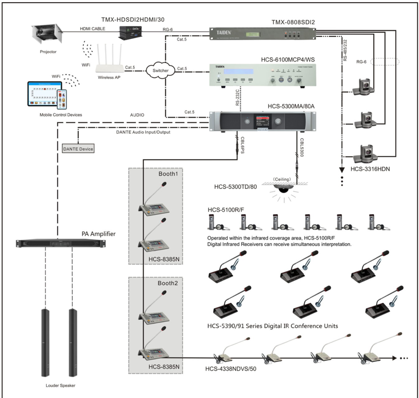
Figure 2.9 System connection [Wired/wireless discussion + digital simultaneous interpretation + voting + video tracking]
