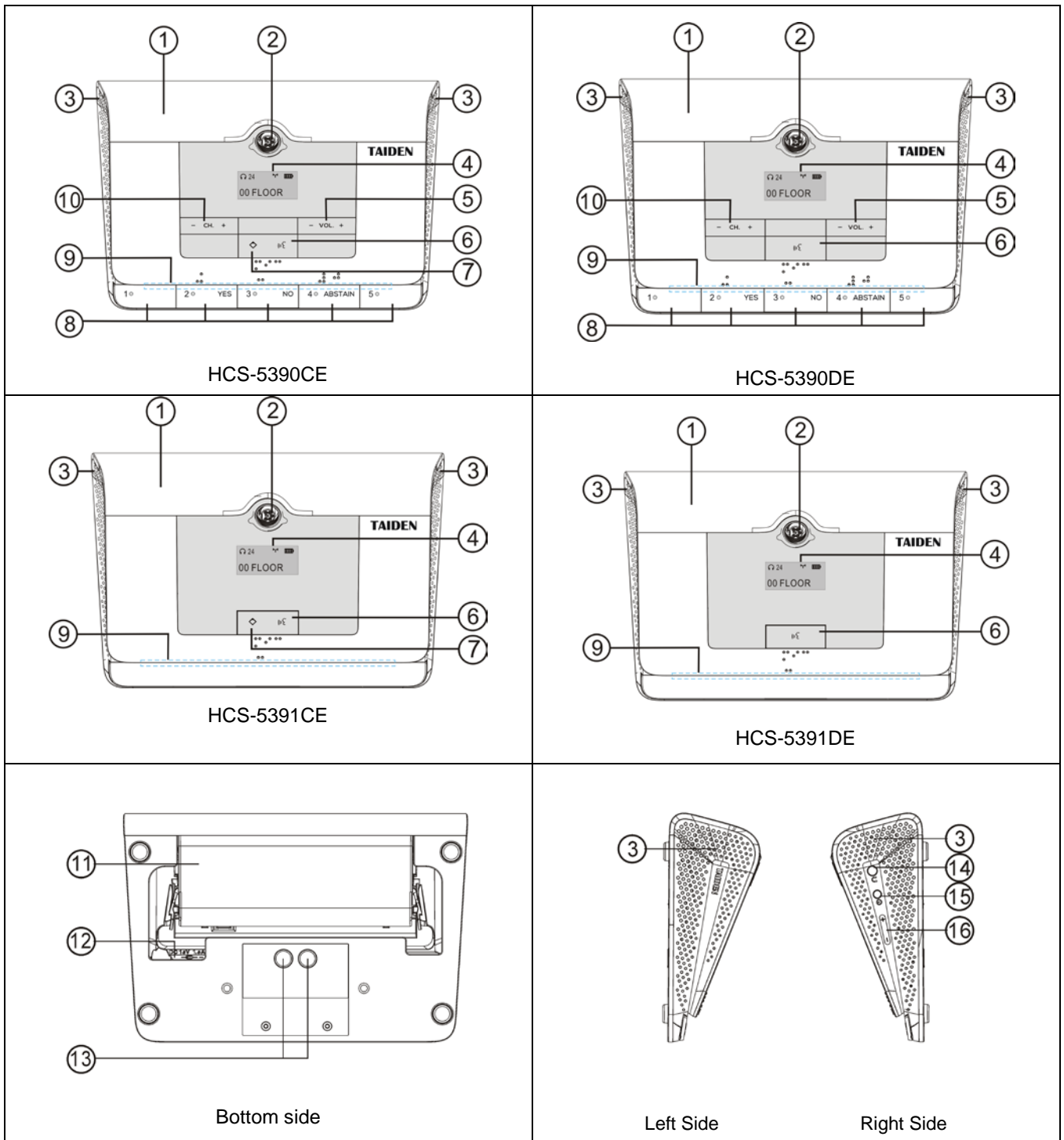
Figure 4.21 HCS-5390 series digital infrared wireless conference unit
