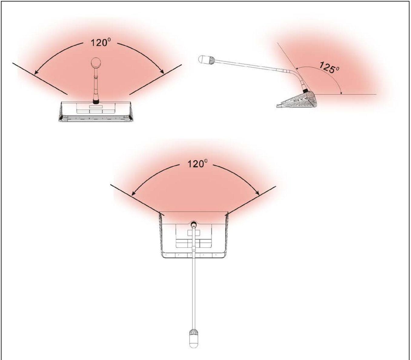
Figure 4.22 Coverage area of new generation digital infrared wireless conference unit
