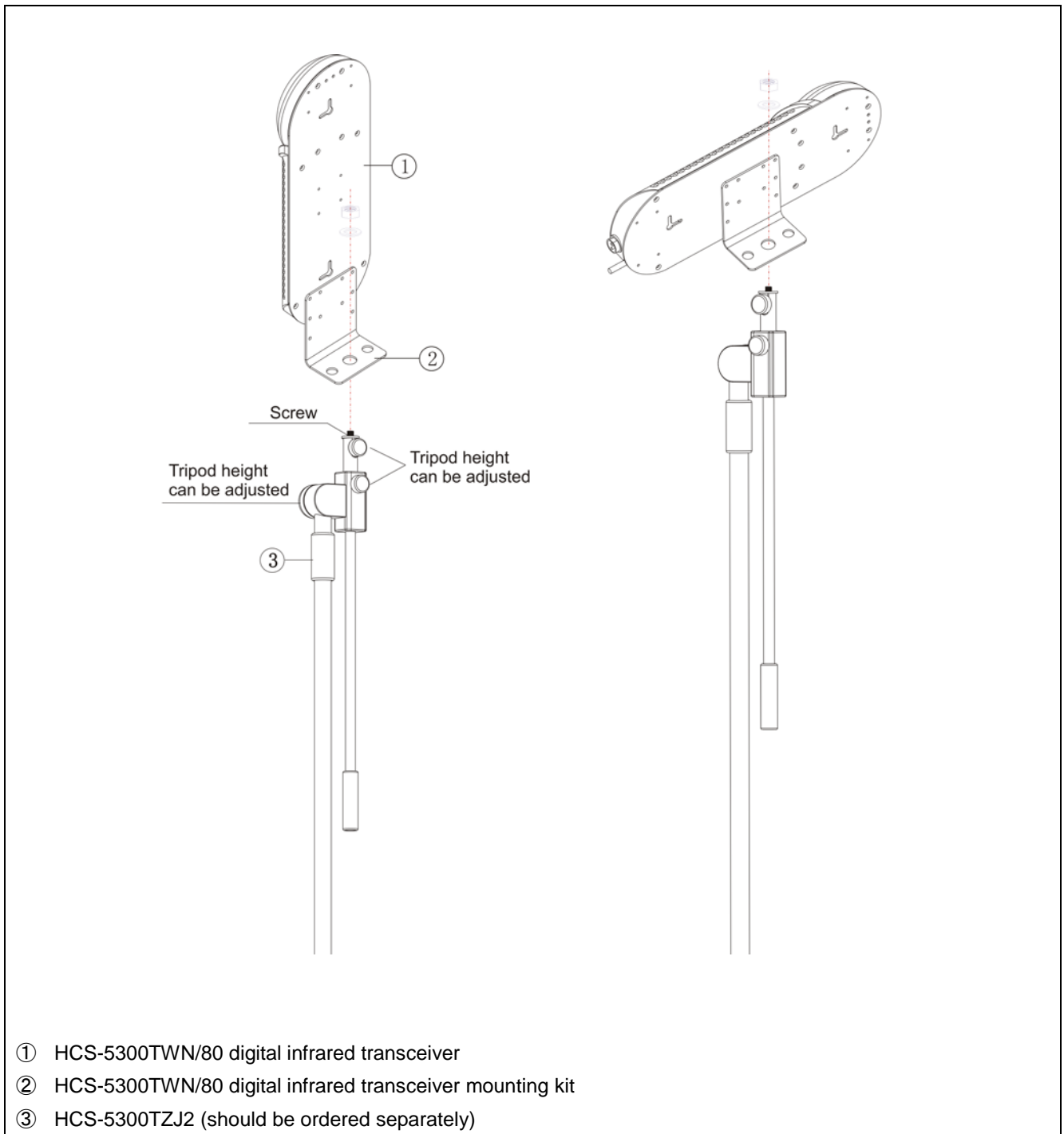
Figure 3.32 HCS-5300TWN/80 digital infrared transceiver tripod mounted
