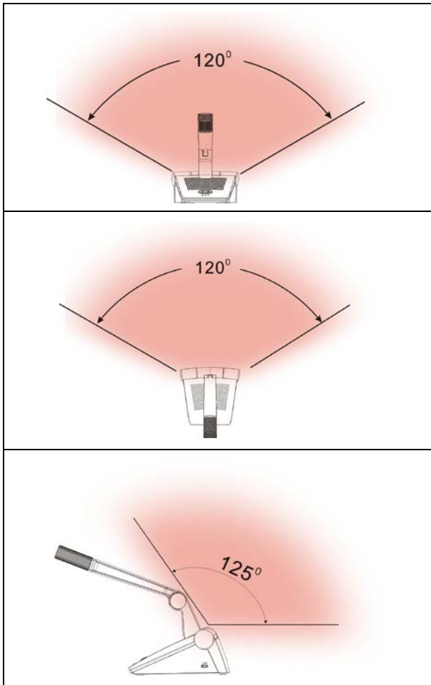
Figure 4.16 Coverage area of digital infrared wireless conference unit
