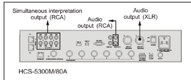
Figure 2.7 Main unit connecting to recording device
