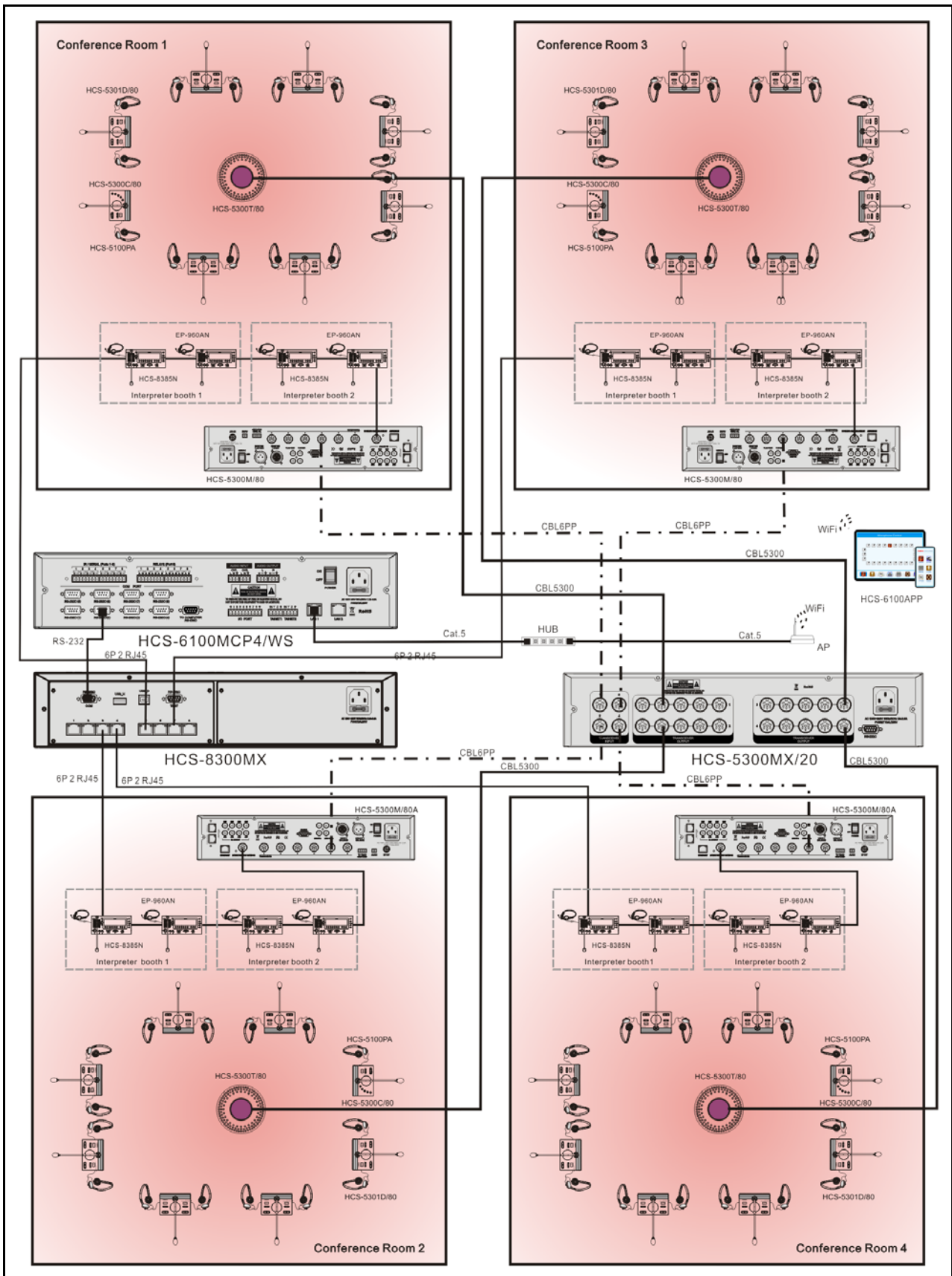
Figure 6.6 Conference rooms combination 2
