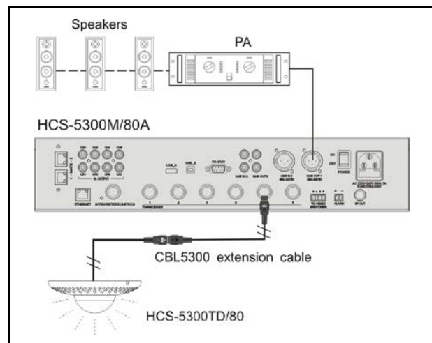
Figure 2.8 Digital infrared wireless conference main unit connecting to PA
